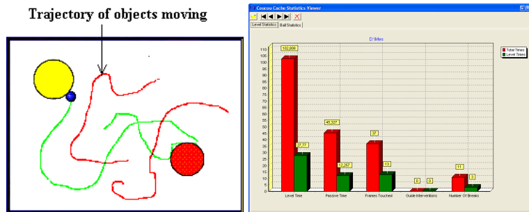
Fig. 3. Execution trace
