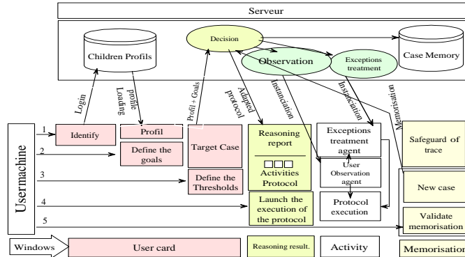
Fig. 4. Implementation
