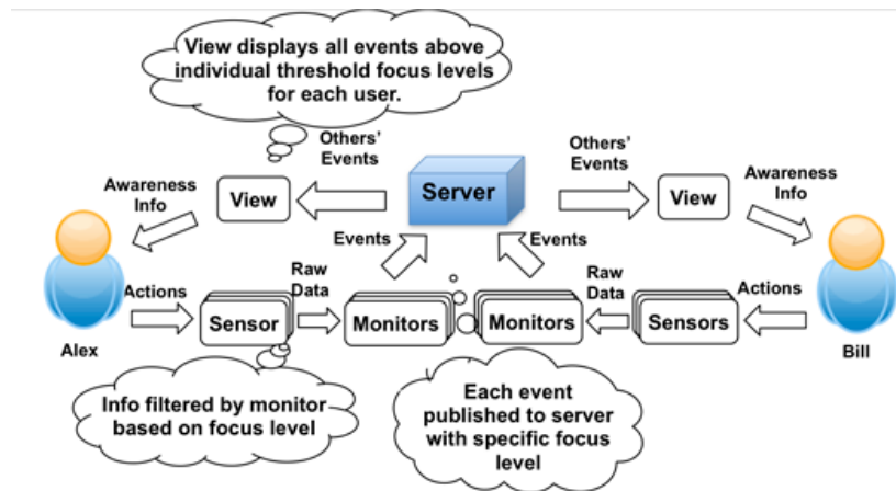
Figure 1. Information flow in the OpenMessenger Framework
