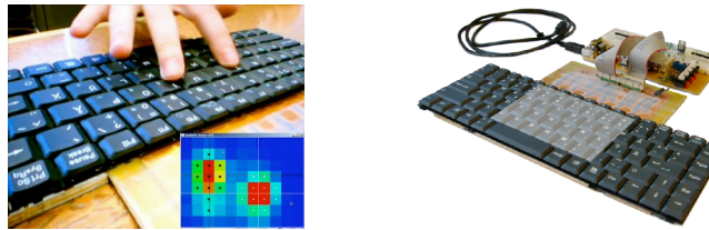
Fig. 1. Left: Color value map and finger position on the keyboard. Right: DGTS electronics.
