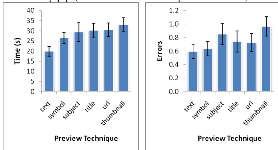
Fig. 3. A) Mean time ( \pm SE) per task by preview technique; B) Mean errors ( \pm SE) per task by preview technique
