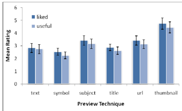
Fig. 4. Mean ratings ( \pm SE) for how liked and how useful the preview techniques were on a 5-pt scale (lower rating = more liked and more useful)
