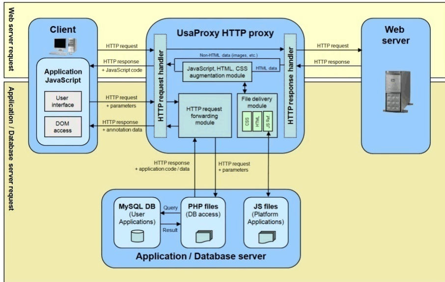
Fig. 1. Components of a proxy-based application platform: application server, HTTP proxy and client side JavaScript. With this approach, no installation of software is necessary on the client browser or the web server.
