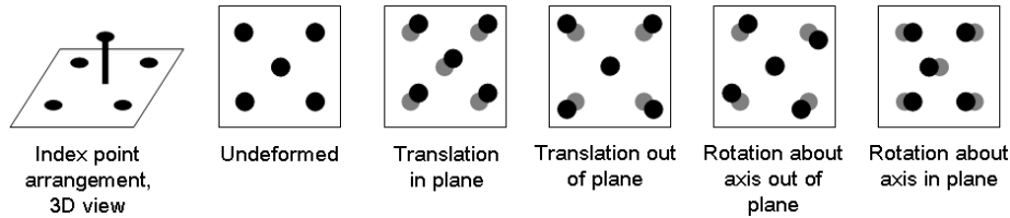
Fig. 2. Arrangement of index points and 6DOF decoding of translations and rotations.
