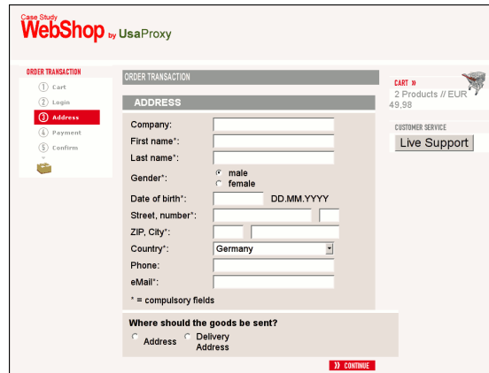
Fig. 5. On the example website, visitors can request immediate help using the “Live Support” button. From that moment, their mouse movements and other actions on the page become visible to the website’s live support staff.
