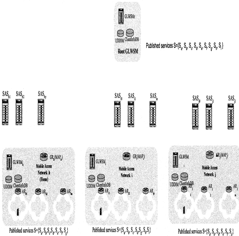
Figure 2. GLWSA topology
