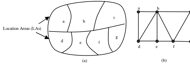
Fig.2. (a) Regional map with LAs (b) Graph model showing the interconnections of LAs
