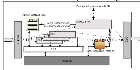
Fig. 4. Active Node Architecture
