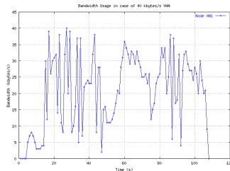
Fig. 6. Bandwidth usage at AN1
