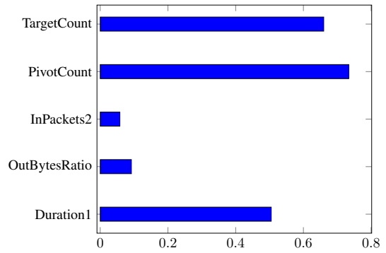
Figure 2. Bar Chart Showing Pearson Linear Correlation Coefficient Between Suspicious Label and Attributes.
