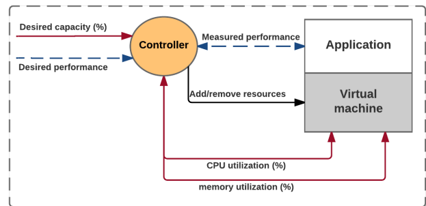
Fig. 1: Capacity- and performance-based controller
