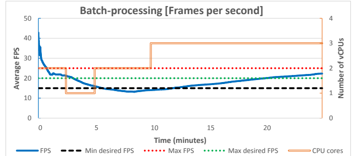
Fig. 10: Batch-processing: FPS in relation to vCPUs
