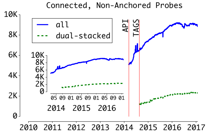
Fig. 4. Evolution of connected dual-stacked probes. The plot is generated using the probe archive API [1] which provides probe metadata since March 2014. The API reports probe tags starting August 2014. Around 25.99% (2301 / 8855) of all connected non-anchored probes are dual-stacked as of Jan 2017.
