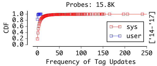
Fig. 14. Frequency of tag changes over time. \sim 2.8\% of probe hosts ever update their user tags. On the other hand more than half of the probes ( \sim 61.4\% ) received at least one update on system tags with \sim 13.1\% of probes receiving at least 10 updates. Whenever user tags are changed, more tags are added / deleted (upto 7 tags changed at once) when compared to system tags.
