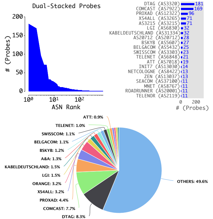
Fig. 8. AS-based distribution of dual-stacked probes. The plot is generated using the RIPE Atlas Probe API [4]. The ASNs are ranked by the number of deployed probes. A large number (822) of ASNs are covered by dual-stacked probes. The entire list is made available at: http://goo.gl/bR5JEd .
