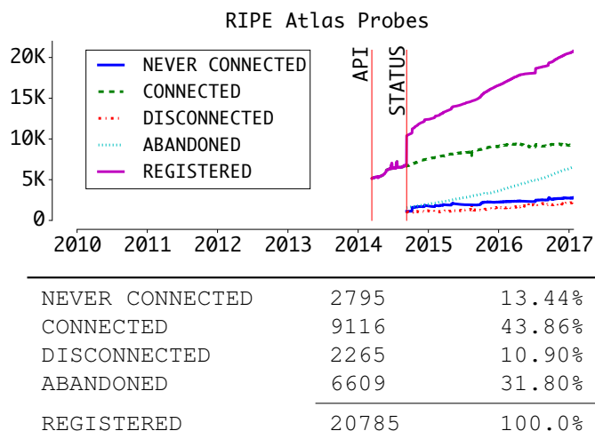
Fig. 1. Evolution of RIPE Atlas probes by their connection status. The plot is generated using the probe archive API [1] which provides probe metadata since Mar 2014. The API was updated to also report the status information of each probe starting Sep 2014. ~9.1K probes are connected out of ~20.7K registered probes as of Jan 2017.
