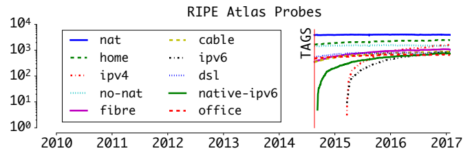
Fig. 13. Time series of top 10 user tags sorted by the number of connected probes. Popular user tags are centered around home probes.
