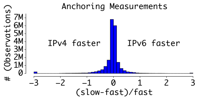
Fig. 11. 5 th percentile comparison of latencies over IPv4 and IPv6 from 2941 RIPE Atlas probes to 149 RIPE Atlas anchors using a month-long (Sep-Oct 2015) dataset consisting of 20M data points. The latencies appear comparable, although IPv4 tends to show marginally better performance. The raw dataset is available at: http://goo.gl/dOJL5Q
