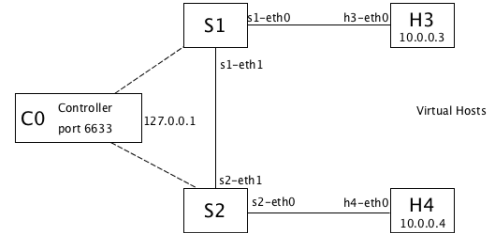
Fig. 2. Controller Performance Experiment Topology
