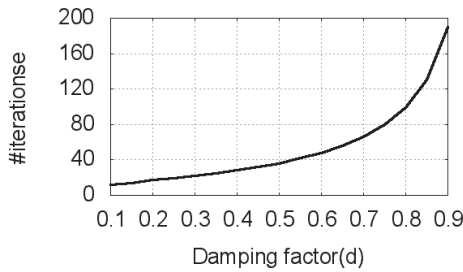
Fig. 11: Number of PageRank iterations
