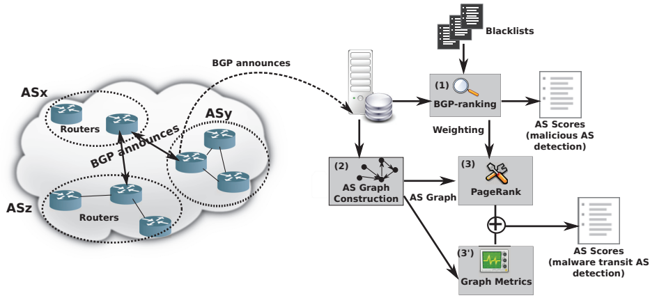
Fig. 1: Information flow and processing of ASMATRA
