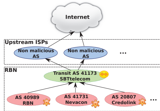
Fig. 2: Overview of the Russian Business Network (RBN)
