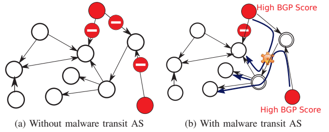
Fig. 4: De-peering known malicious ASs
