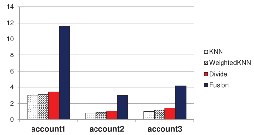
Fig. 12: Overall Score for K = 20 , k = 5
