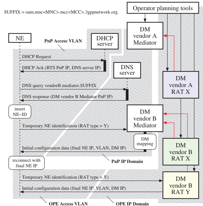
Fig. 3. Initial connectivity sequence, showing the infrastructure of two vendors co-existing in a multi-vendor deployment.
