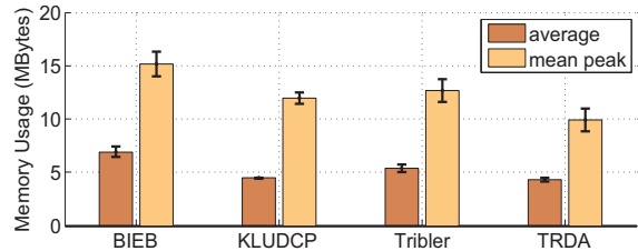
Fig. 8. Memory consumption during playback of video with size 235 MB
