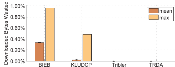
Fig. 7. Amount of wasted data downloaded but discarded during playback
