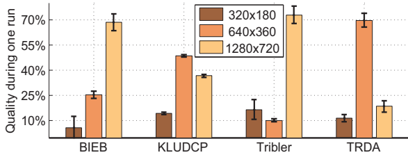
Fig. 5. Playback Quality in terms of segments per representation
