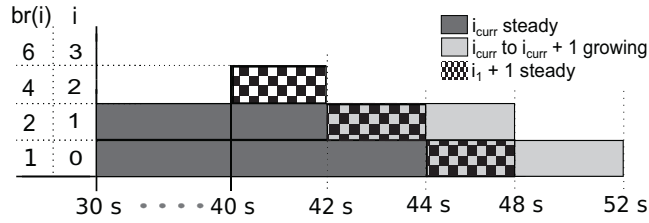
Fig. 1. Example for steady phase Q1, Q2 and growing phase from Q1 to Q2
