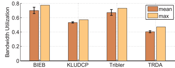
Fig. 6. Bandwidth utilization compared to the theoretical maximum
