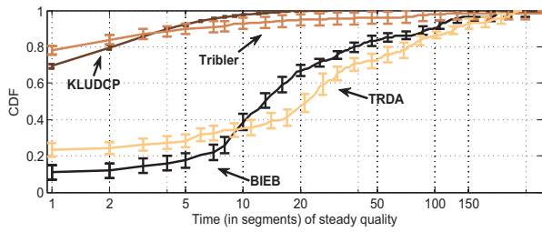
Fig. 3. Inter Switching Times CDF
