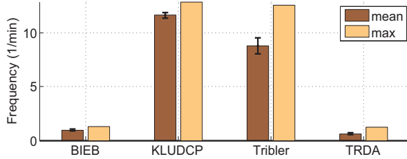
Fig. 4. Frequency of quality switches during playback
