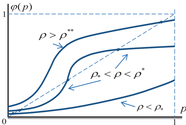
Figure 1. Solution of the fixed-point equation (6)
