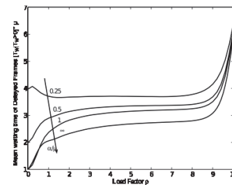
Fig. 2b. Different Overhead Loads versus Load Factor \rho
