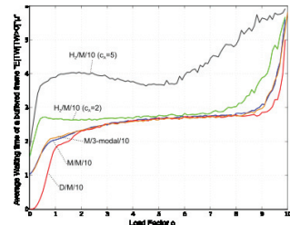
Fig. 1e. Simulation Results: Influence of Interarrival Time and Realistic Service Time DF
