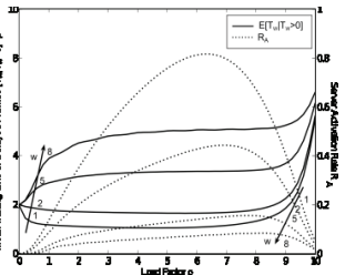
Fig. 2a. Mean Waiting time of Delayed Frames and Server Activation rate versus Load \rho
