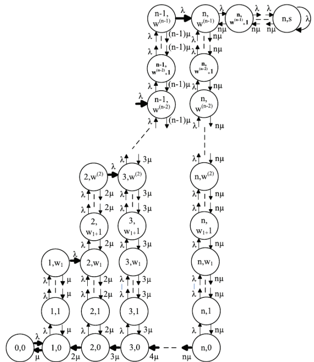
Fig. 2. State Transition Diagram for the Multiple Parallel Hystereses Model
