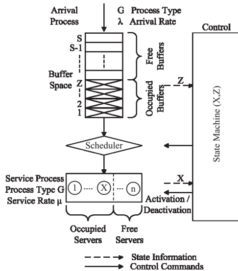
Fig. 1. Generic Model for Dynamic Activation/Deactivation of Servers Parameters: n =total number of servers, s =total number of frame buffers \lambda = arrival rate of frames, \mu = service rate of a server
