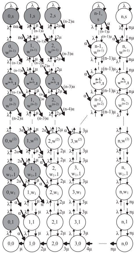
Fig. 3. State Transition Diagram for the Multiple Parallel Hysteresis Model with Activation Overhead
