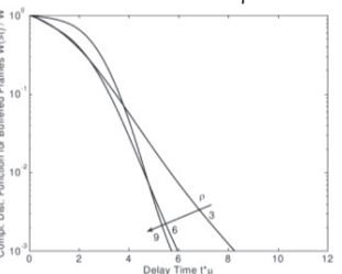
Fig. 1d. Comp. Distribution Function for Waiting Times of Buffered Frames
