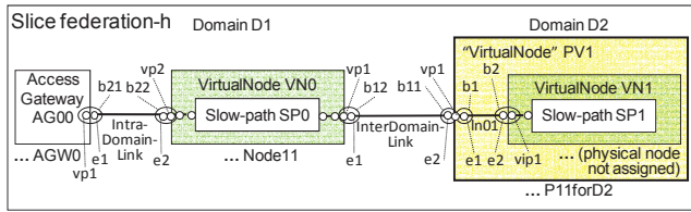
(a) Slice specification given to domain 1
