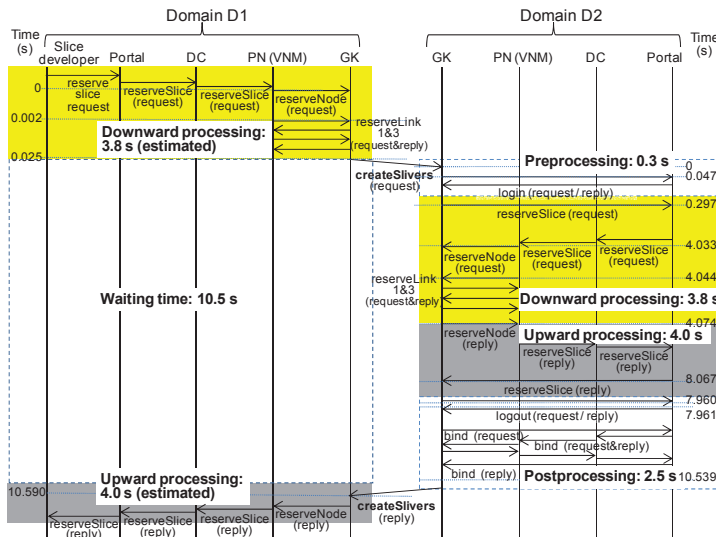
Figure 9. Measurement of slice creation
