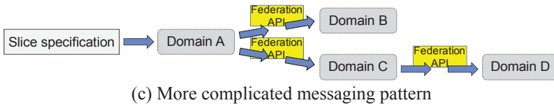
Figure 3. Federation API and cross-domain slice creation
