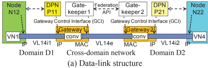
(a) Data-link structure (b) Data communication using arbitrary packet-format Figure 6. Inter-domain data-link structure and data communication
