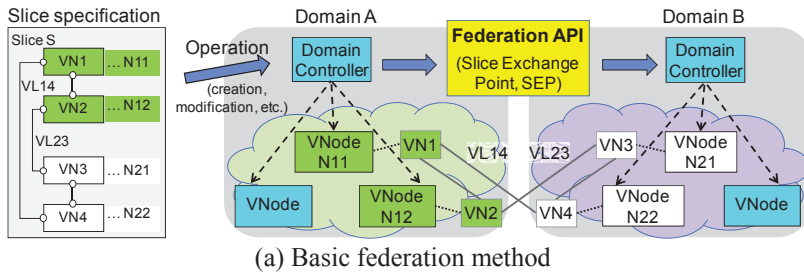
(a) Basic federation method
