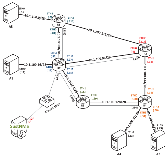
Fig. 3. Network topology equipped with the evaluation test environment described in Section IV-A
