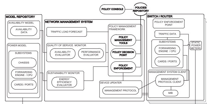
Fig. 1. SustNMS Architecture [5]
