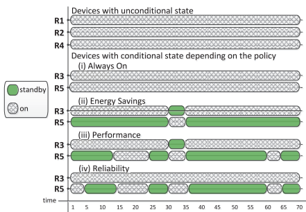
Fig. 6. Topology changes applied by the SustNMS. Probe rate of 1 min.
