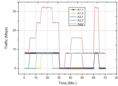
Fig. 4. Traffic profile
