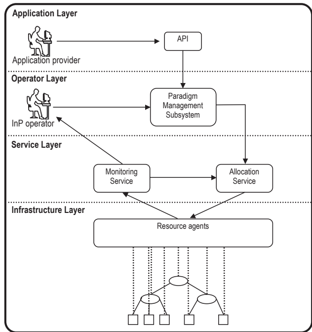
Fig. 3. Architecture of a paradigm-based provisioning system
