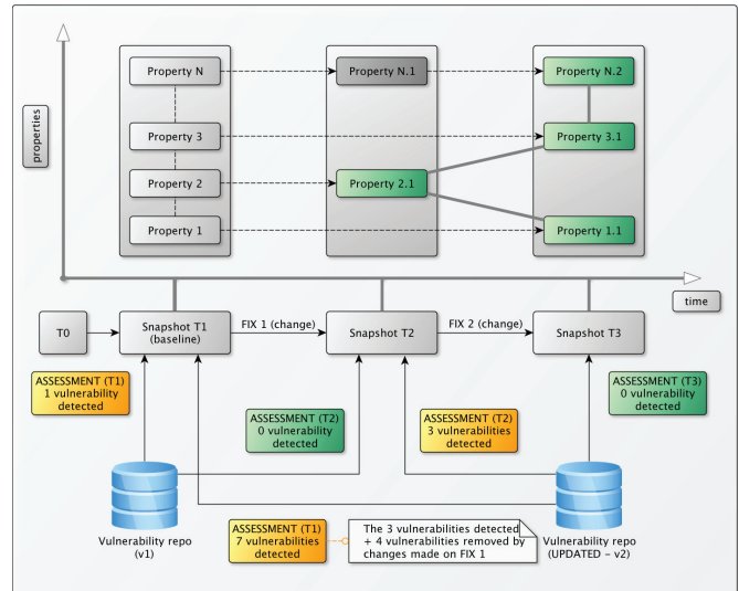
Fig. 3: SVN-based assessment
