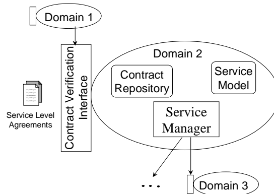
Figure 2. Federation Architecture
