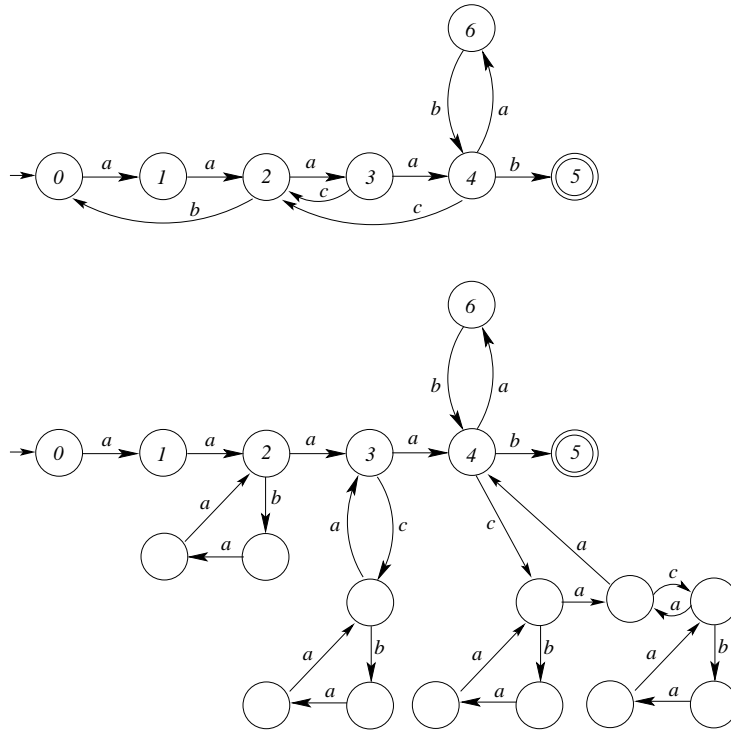
Fig. 2. A 1cfd (up) and the corresponding balloon automaton (down).
