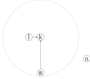
Fig. 1. Connectivity example.
