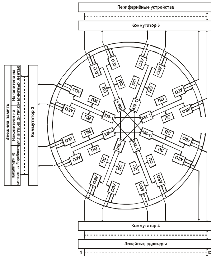
Figure 5. Structure of 16-processor variant CAC “Svjaz-1”
