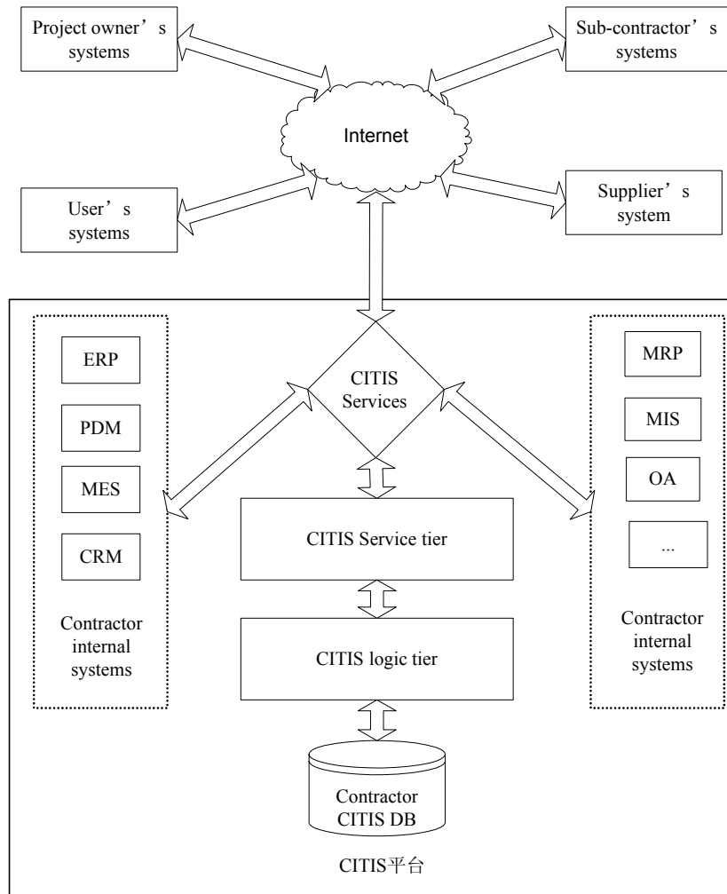
Figure 1. The SDEP's System Architecture
