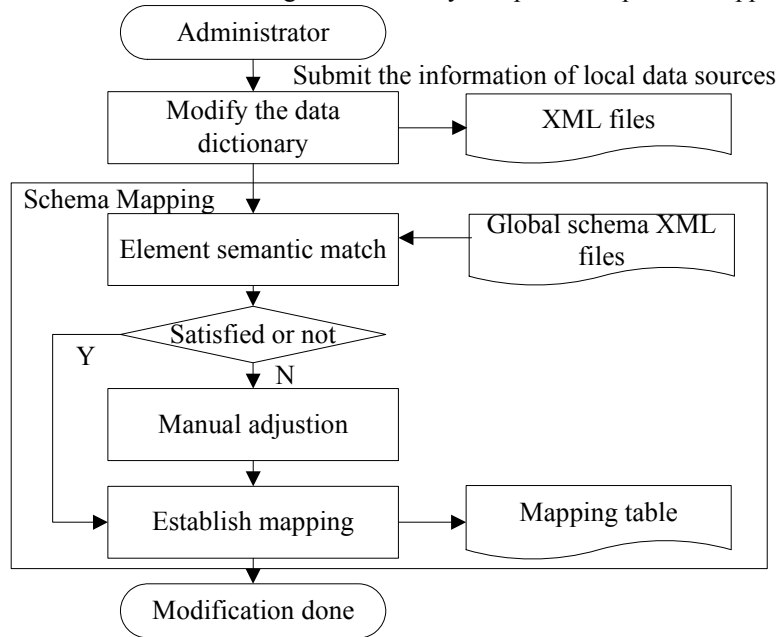
Figure 3. Schema Modify Flowchart
