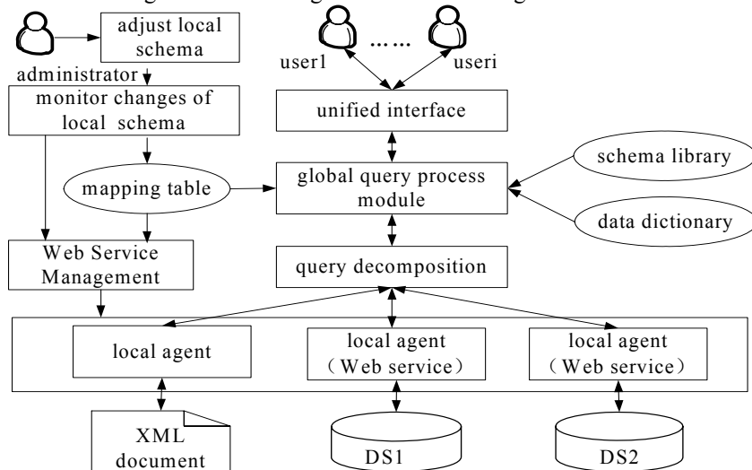
Figure 1. The Framework of Self-Adaptive Heterogeneous Data Integration System
