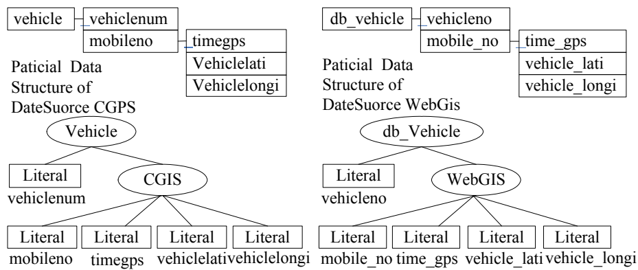
Figure 2. XML Schema Structure for Part of Data Source and their Ontology Structure
