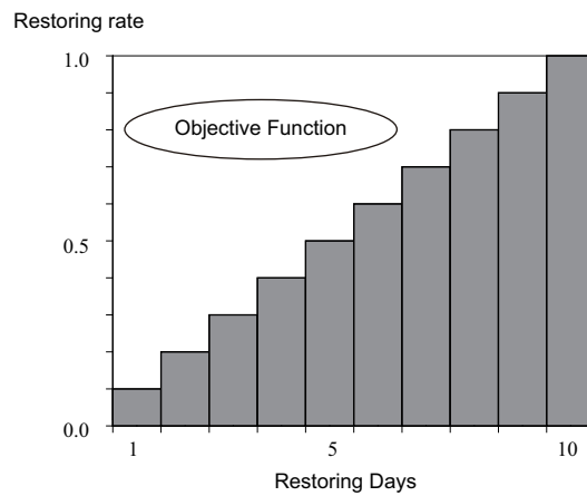
Fig. 16 Objective function
