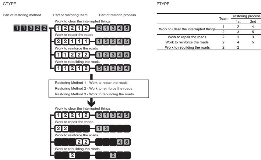
Fig. 18 DNA structure
