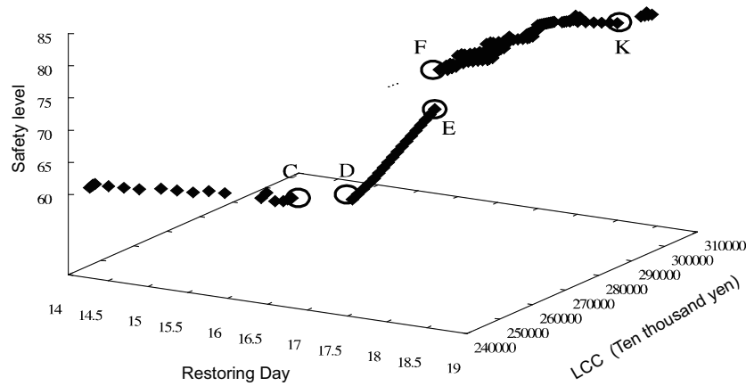
Fig. 22 Pareto solutions obtained by MOGA
