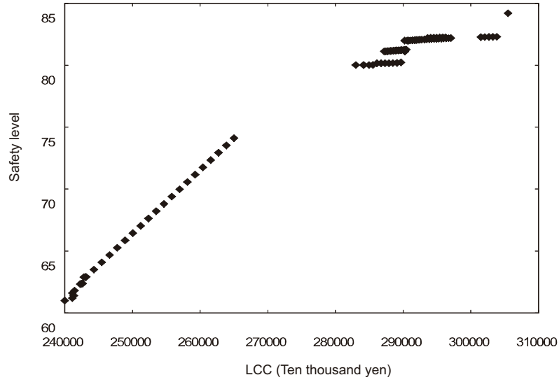
Fig. 25 Relation between LCC and safety level
