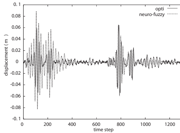
Fig. 4 Experiment result of adaptive controller
