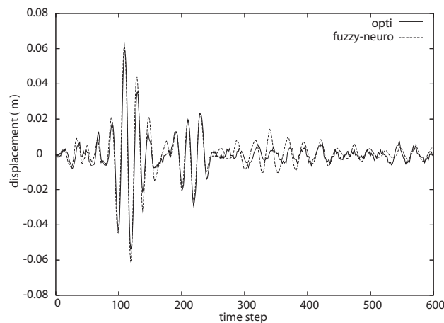
Fig. 3 Experiment result of robust controller
