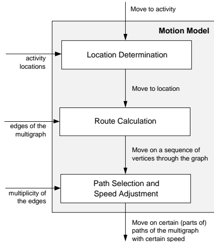
Fig. 3. The three layers of the motion model. In the location determination layer , a suitable location for a given activity is selected. After that, the route calculation determines a sequence of intermediate vertices to reach that location. Finally, the lowest layer performs a path selection and speed adjustment step to handle effects of crowded paths and slower moving pedestrians.
