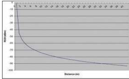
Fig. 1. Ideal RSSI values (on equation 1, A=40 , n=3 )
