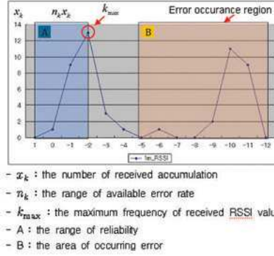
Fig. 4. The variation of RSSI values at indoor environment in 1m; it illustrates the RSSI values with k_{max} of suggested filtering method
