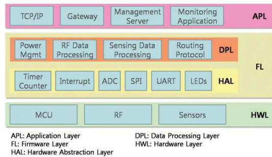
Fig. 8. The structure of Firmware
