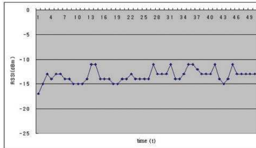
Fig. 2. The variation of RSSI values in terms of received time at outdoor environment in 1m.
