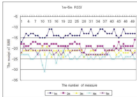
Fig. 9. The variation of RSSI value in 1-5m
