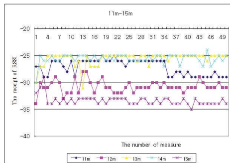
Fig. 11. The variation of RSSI value in 11-15m
