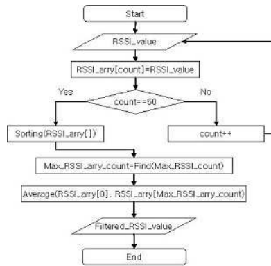
Fig. 5. The flow chart of suggested filtering g algorithm
