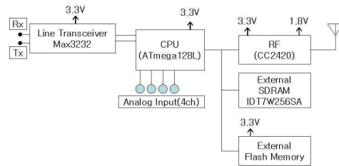
Fig. 7. Structure of main module
