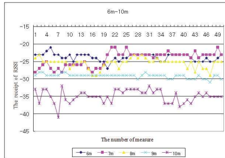
Fig. 10. The variation of RSSI value in 6-10m
