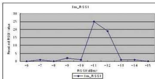
Fig. 3. The frequency of distribution curve of RSSI values at outdoor environment in 1m.
