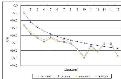
Fig. 12. Comparing the suggested RSSI value
