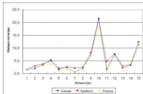
Fig. 13. Comparing distance error with converted RSSI
