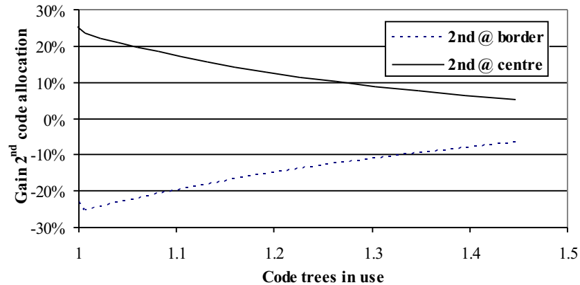
Fig. 5. Capacity gain for code allocation strategies
