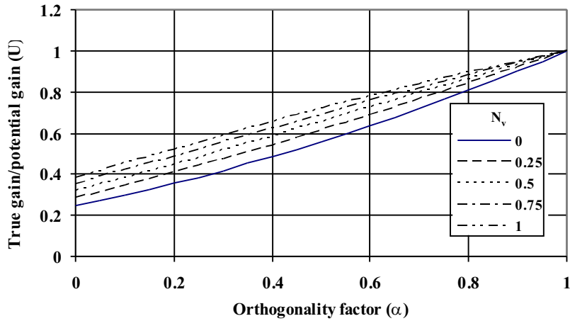
Fig. 3. Usability of the capacity gain on secondary scrambling code
