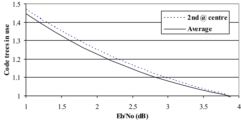
Fig. 6. Effective capacity for code allocation strategies
