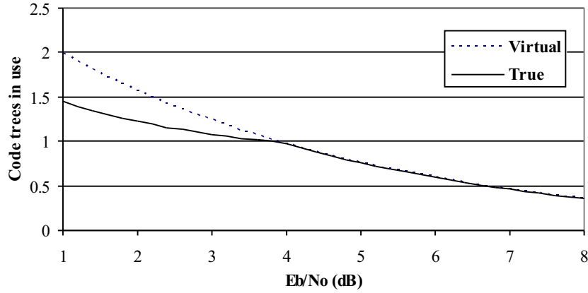
Fig. 2. Capacity impact of secondary scrambling code
