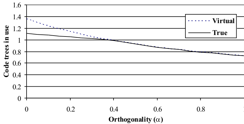
Fig. 4. Capacity impact of orthogonality
