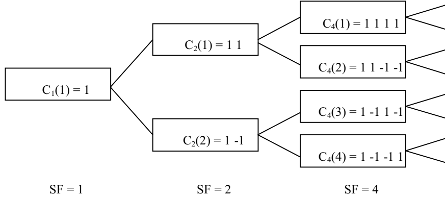
Fig. 1. OVVSF channelization code tree [1], [2]
