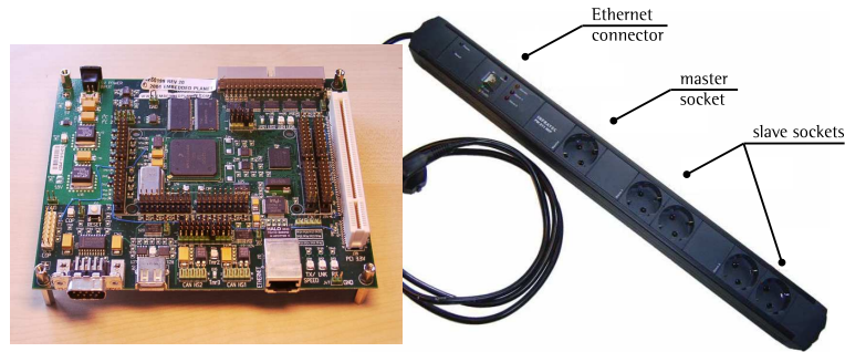
Fig. 2: Left: The EP5200 board is based on an PowerPC-603 processor. It has no moving parts. The flash memory can be used to host the root file-system. Right: The Ethernet-capable multiple plug is an important actuator for controlling all kinds of devices which can be switched on and off only.
