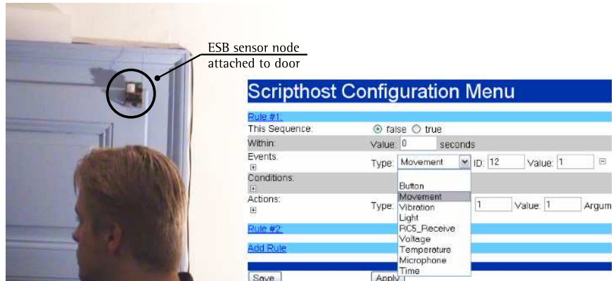
Fig. 3: Left: Extract from our demo video: Two sensor readings are used to distinguish whether the door is approached from the inside or the outside. Right: Browser-based configuration.
