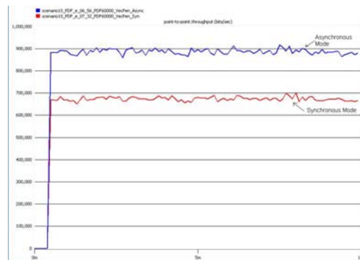
Fig. 6. Asynchronous/Synchronous Mode Custom PDF model Haptic Traffic Point-to-Point Throughput, Client to Server
