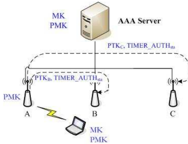
Fig. 6. Distribution of PTKs Keys with IAPP exchanges
