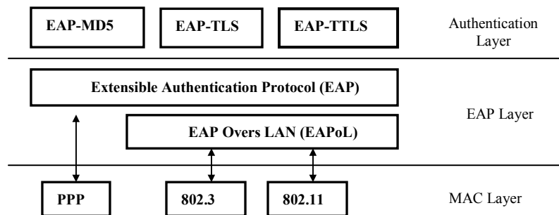
Fig. 1. Authentication Protocols
