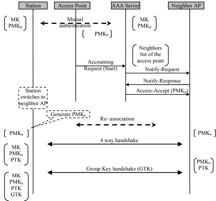
Fig. 3. Pre-authentication exchange with PKD method
