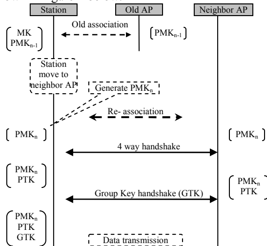
Fig. 4. Re-authentication exchange with PKD
