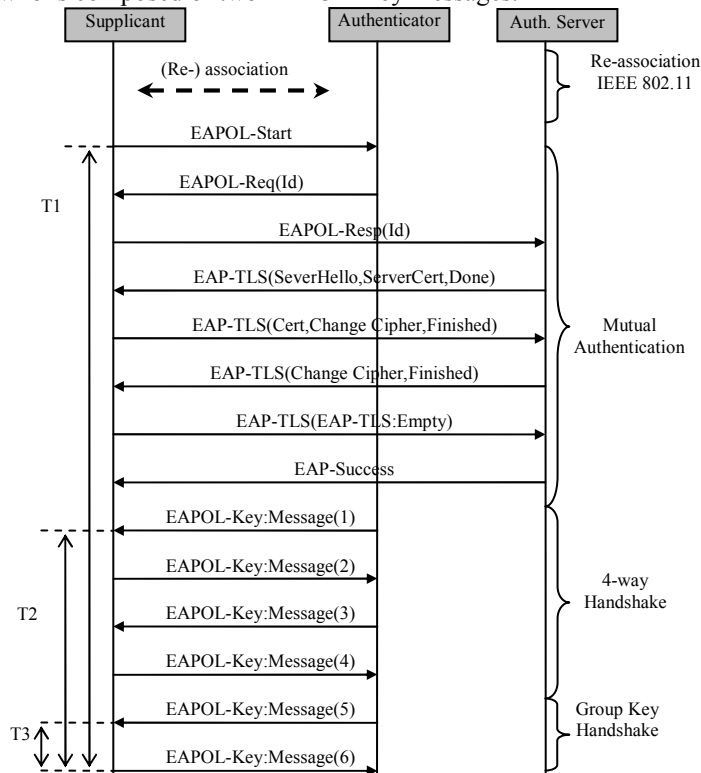
Fig. 2. EAP/TLS Authentication exchange
