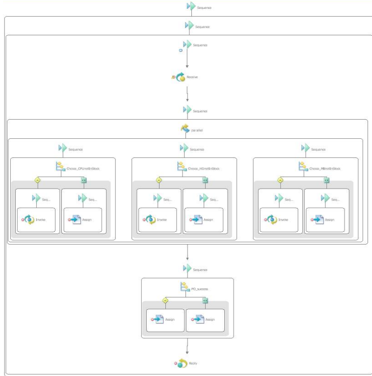
Fig. 5. BPEL process of Manufacturer
