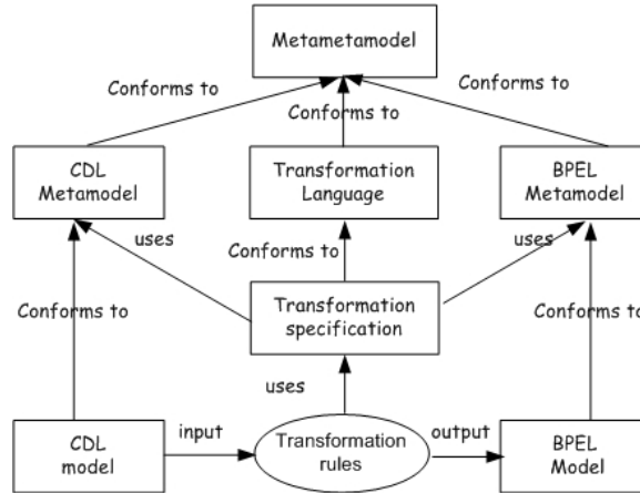
Fig. 2. Model-driven transformation
