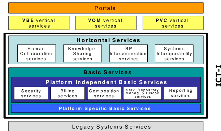
Figure 3 – ICT-I Reference Architecture
