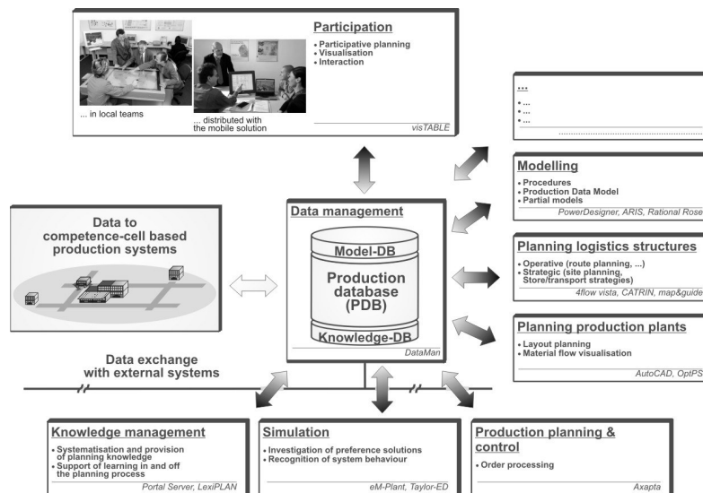
Figure 4 – Net Planning Assistant (Müller et al. 2004)
