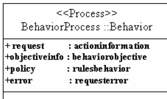
Figure 3 – A UML class used to model a Behavior BPEL Process
