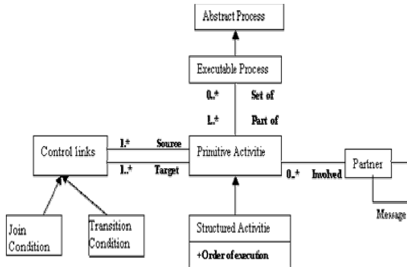
Figure 1 – Model of BPEL Core Concepts
