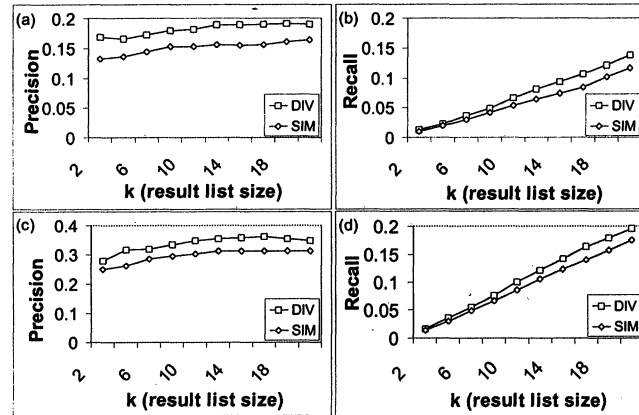
Figure 3. (a) Precision results for the mammals domain, (b) Recall results for the mammals domain, (c) Precision results for the travel domain, (d) Recall results for the travel domain
