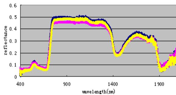
Fig.1 Reflectance spectra of winter wheat leaves
