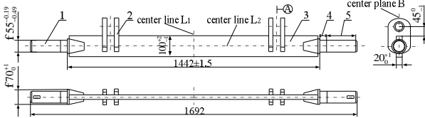
1 end axle; 2 pulling board; 3 brake beam body; 4 sleeve gasket working surface; 5 brake shoe working surface.
