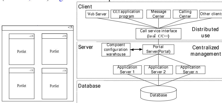
Fig.1. User interface
