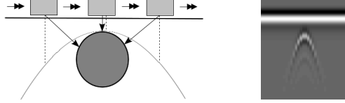
Fig. 1. The antenna (rectangle) is moved perpendicular to the buried object (circle). The downwards directed arrows represent transmitted signals, the dotted lines indicate the position of the received signal values in the corresponding A-Scans. On the radargram (right) one can see a hyperbola branch corresponding to the buried object.
