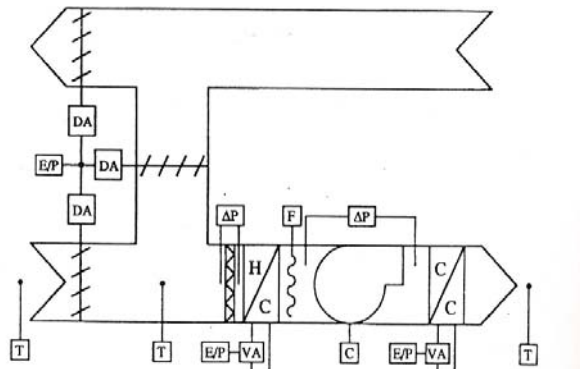
Fig. 2. System Diagram for the Air Handler
