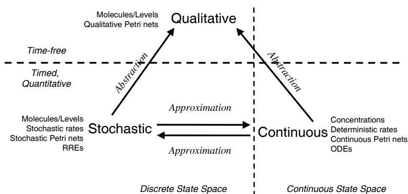
Fig. 3 Conceptual framework of our computational methods.
