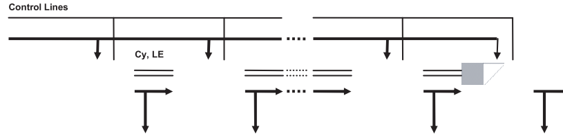
Fig. 6 Insert Sorting circuit block diagram for n-elements.
