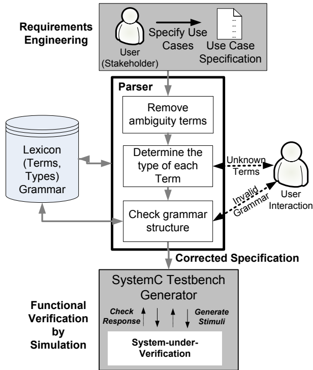
Fig. 1 Novel highly automated approach from textual use cases to a SystemC testbench for functional verification.
